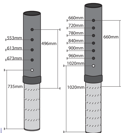
Code 42 Outer: 42mm Dia x 1.6mm RHS Inner: 38mm Dia x 1.6mm RHS Table Height 496 to 735Hmm Counter Height 660mm to 1020mm
