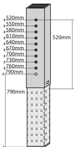
Code 40 Outer: 40mm x 1.6mm SHS Inner: 36mm x 1.6mm SHS 520 to 790Hmm
