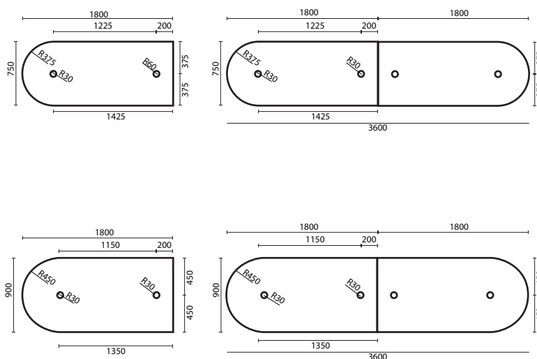
Twelve Student Boardroom Table Created with two 1800x750mm Teknik Tables
